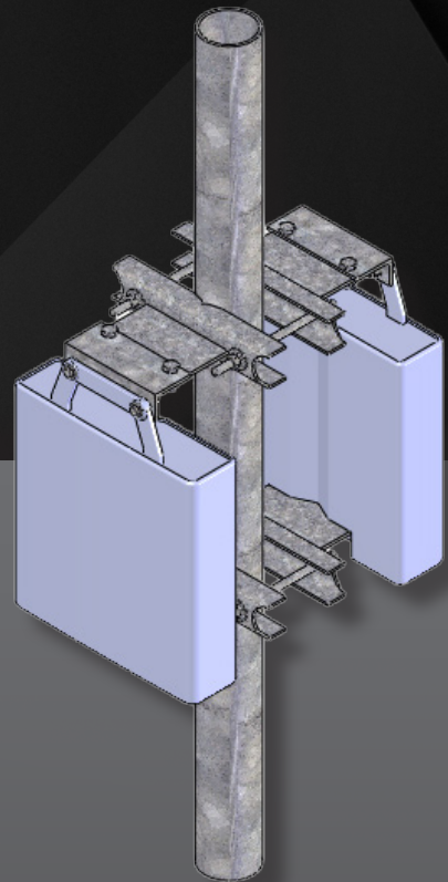
4.927.0063.001 Pipe Mounted
